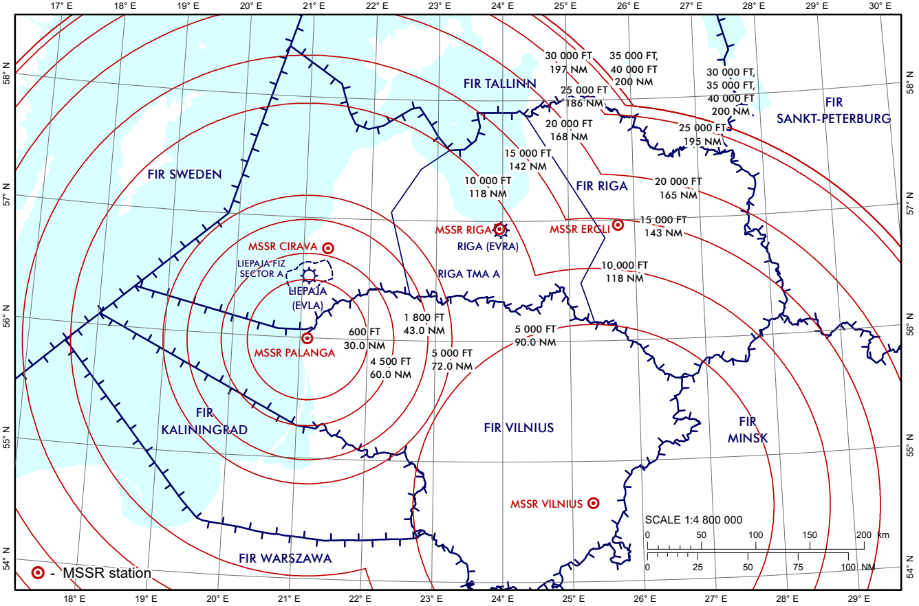
Figure 9 "PALANGA" MODE S MSSR AND "VILNIUS" MODE S MSSR RADARS COVERAGE (VILNIUS FIR/RIGA FIR LAYOUT)
